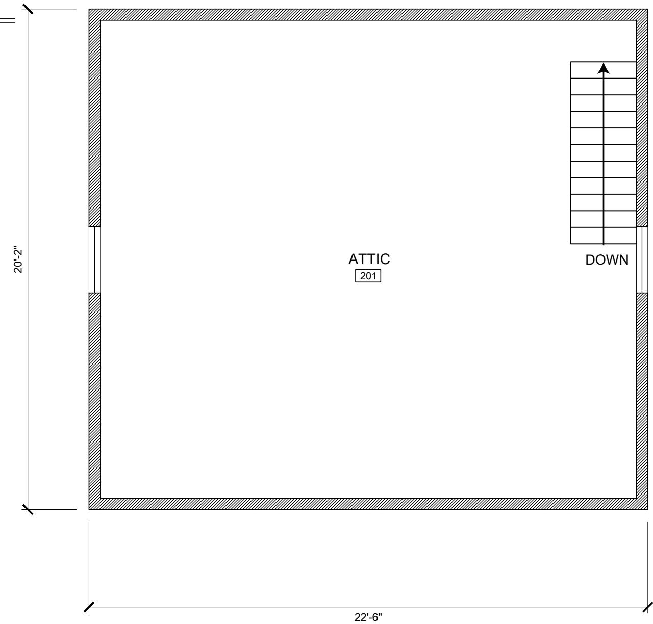
EXISTING ATTIC PLAN - SCALE 1/4" = 1'-0"
