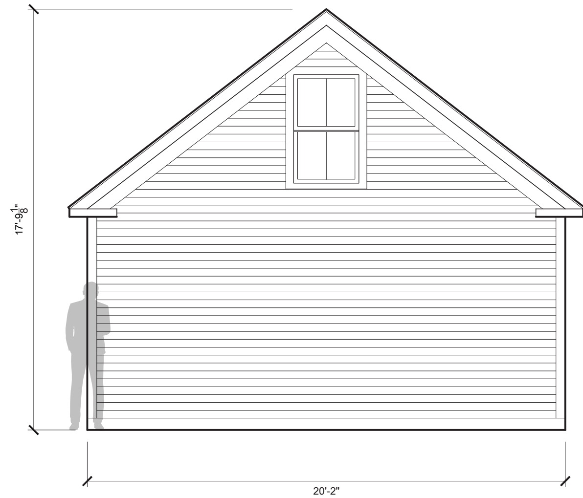
EXISTING ELEVATION (FACING SIDE YARD) - SCALE 1/4" = 1'-0"
