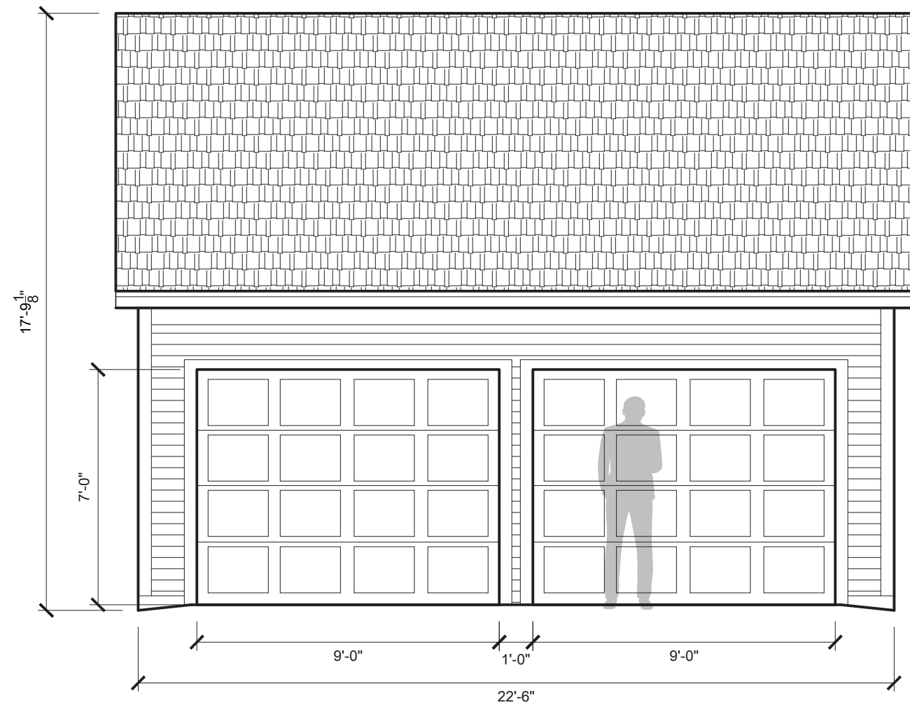
EXISTING ELEVATION (FACING HUBBARD STREET) - SCALE 1/4" = 1'-0"
