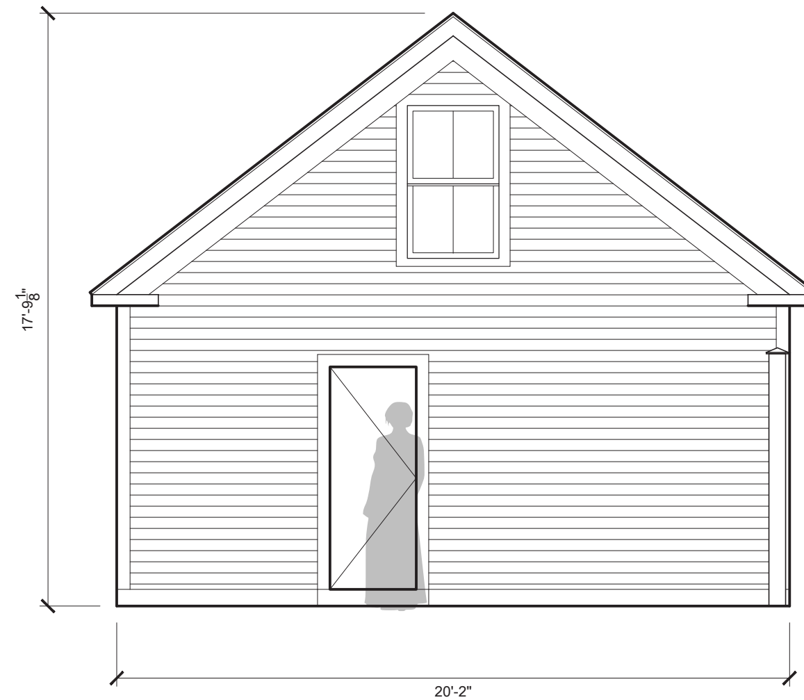
EXISTING ELEVATION (FACING THOREAU STREET) - SCALE 1/4" = 1'-0"
