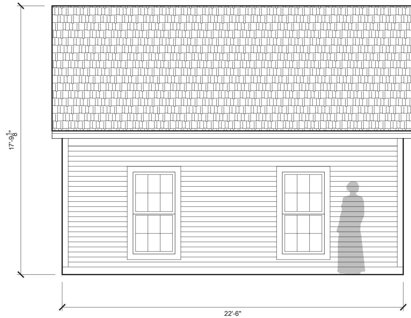
EXISTING ELEVATION (FACING SIDE YARD) - SCALE 1/4" = 1'-0"
