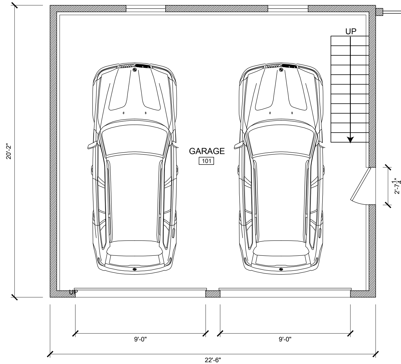
EXISTING GARAGE PLAN - SCALE 1/4" = 1'-0"
