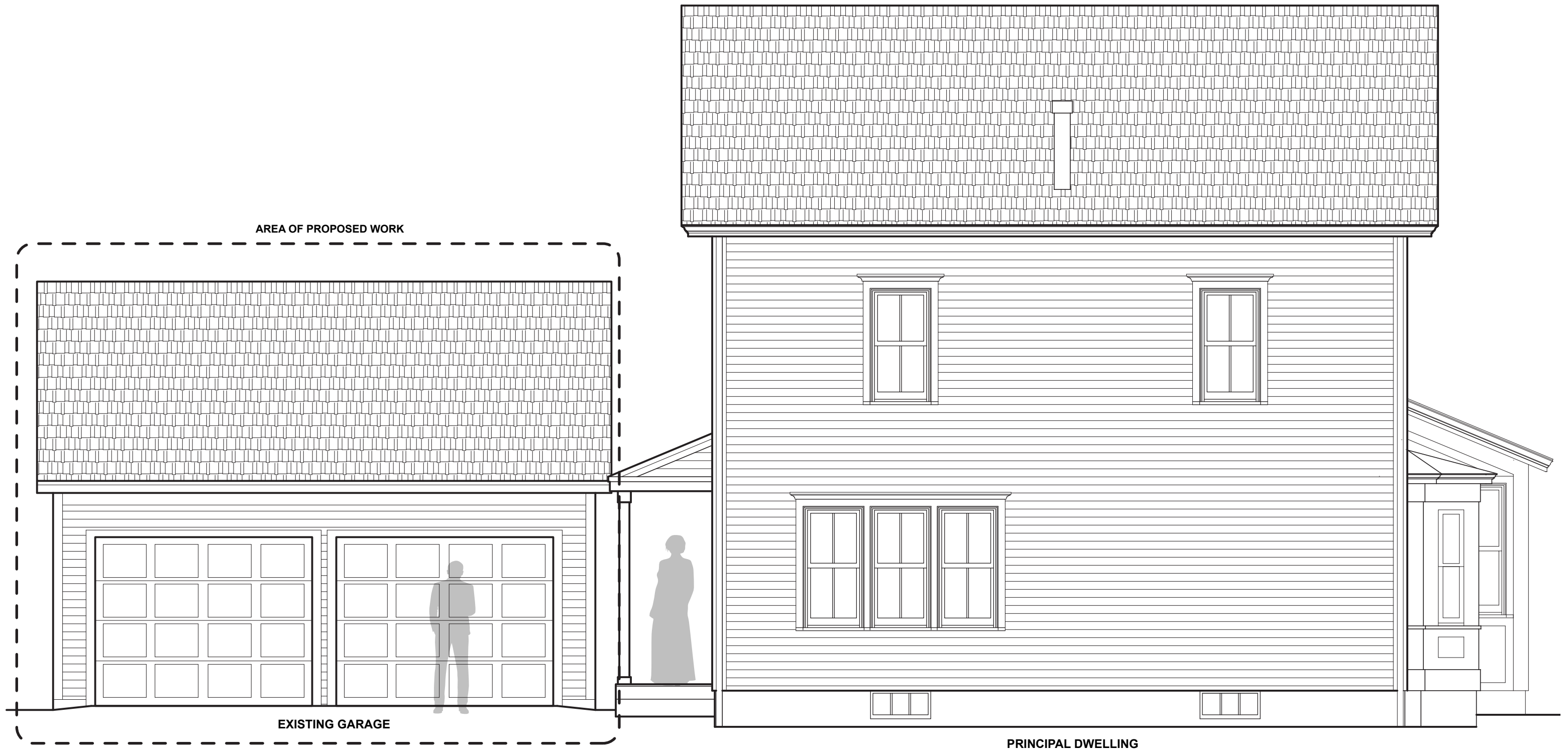
EXISTING ELEVATION (FACING HUBBARD STREET) - SCALE 1/4" = 1'-0"
